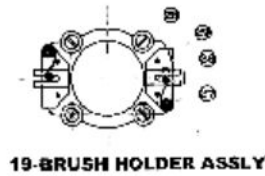
19-BRUSH HOLDER ASSLY.
